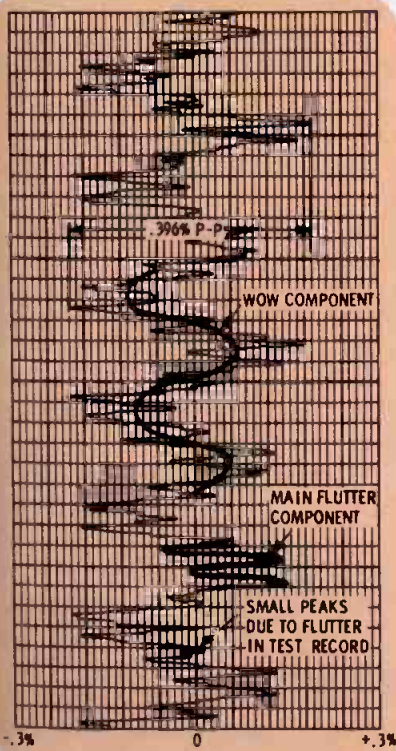
Chart 2. Strip chart recording of wow and flutter from typical turntable. Peak to peak is .396%. NAB weighted measurement was about .06%. This unit was within manufacturer's rated specification, which called for .075% DIN weighted wow and flutter.
